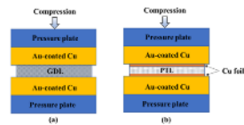
Fig. 1. Illustration of TBC, BCC, and IP-DC measurements for (a) GDLs and (b) PTLs using scanning samples.
